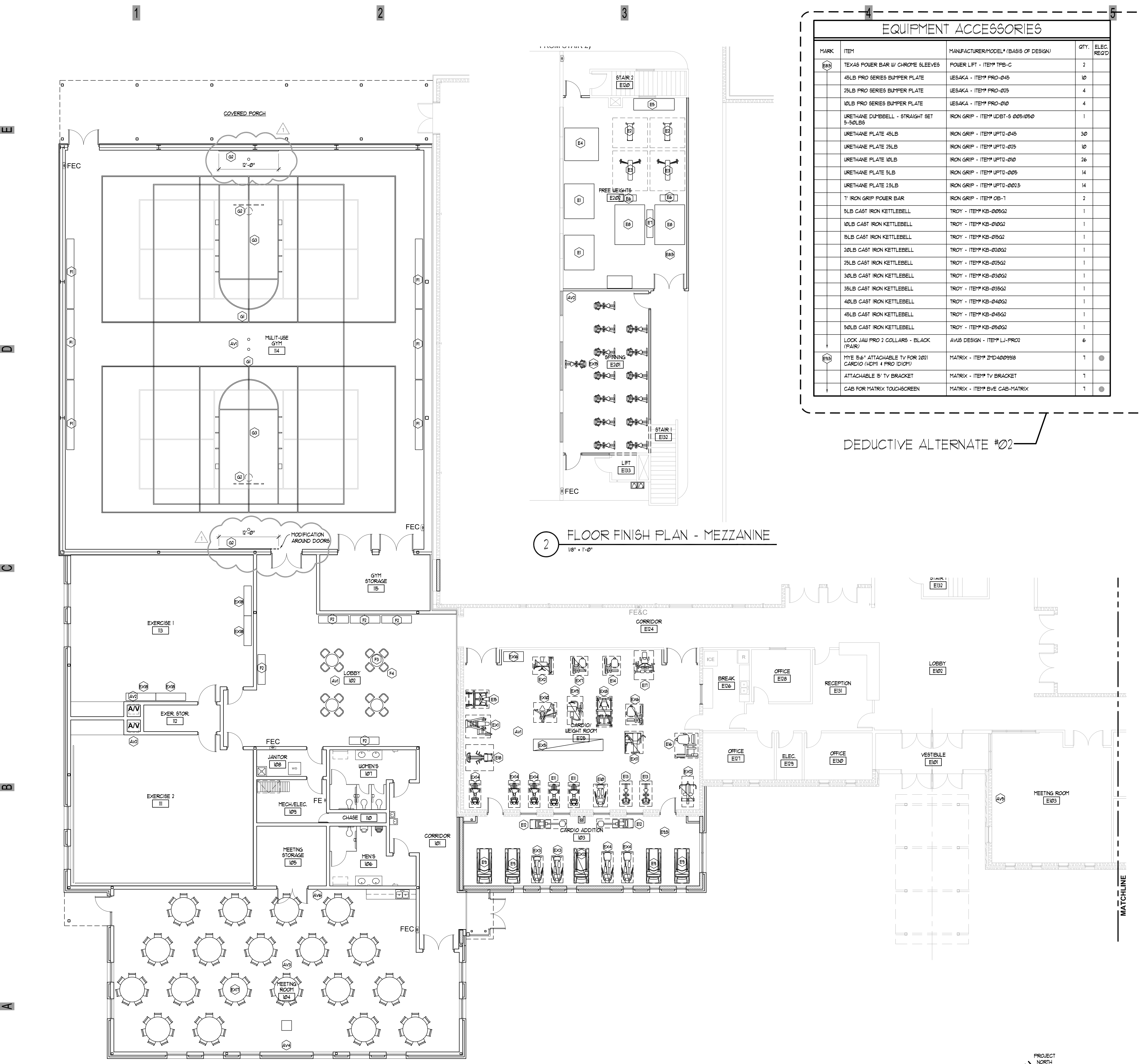
1 FURNITURE PLAN - A 1/8" = 1'-0"
